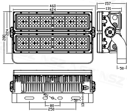
ZY-2097G 400W
