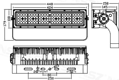
ZY-2097G 200W
