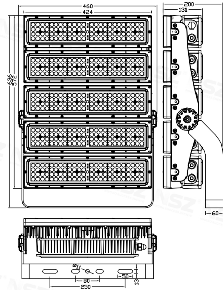
ZY-2097G 1000W
