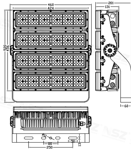
ZY-2097G 800W
