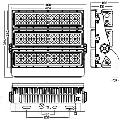
ZY-2097G 600W
